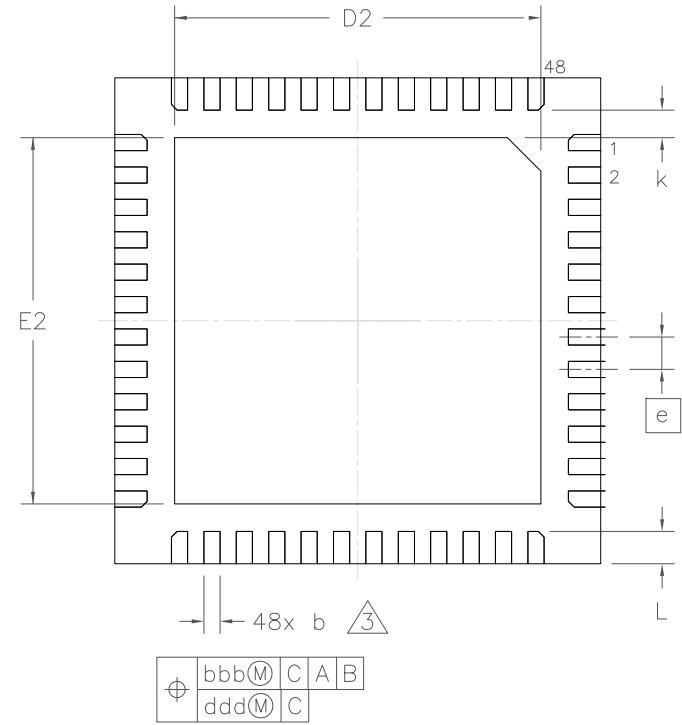
BOTTOM VIEW PACKAGE FLIPPED LEFT TO RIGHT
